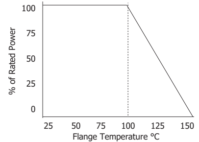
T50R0-40-16X Power Derating Curve
