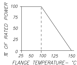
DERATING CURVE:
