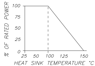
DERATING CURVE:
